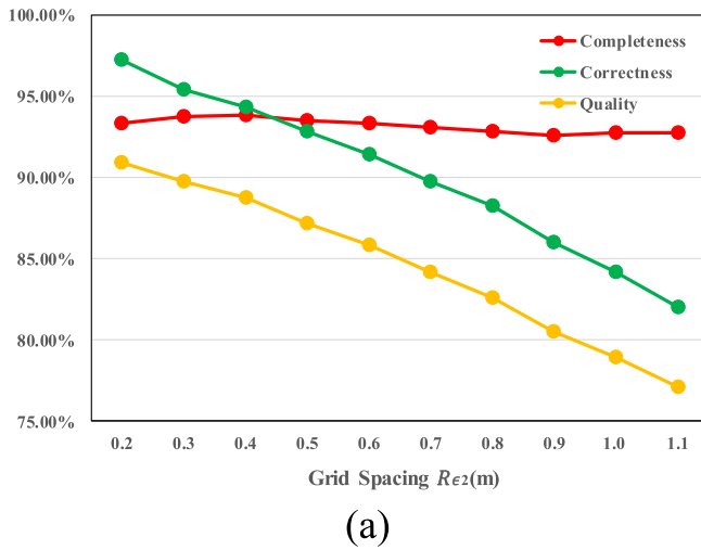
Fig. 8. Illustrations of the performance of erroneous boundary removal and CNN-based completion under different grid spacing: (a) Completeness, correctness, and quality results. (b) Time cost.
