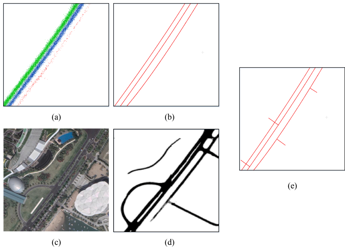
Fig. 13. Road centerline extraction. (a) Taxi GPS trajectory points. (b) Road centerlines obtained from taxi GPS trajectory points. (c) Remote sensing image. (d) Roads extracted from image (c). (e) Final road centerlines merged from (b) and (d).
